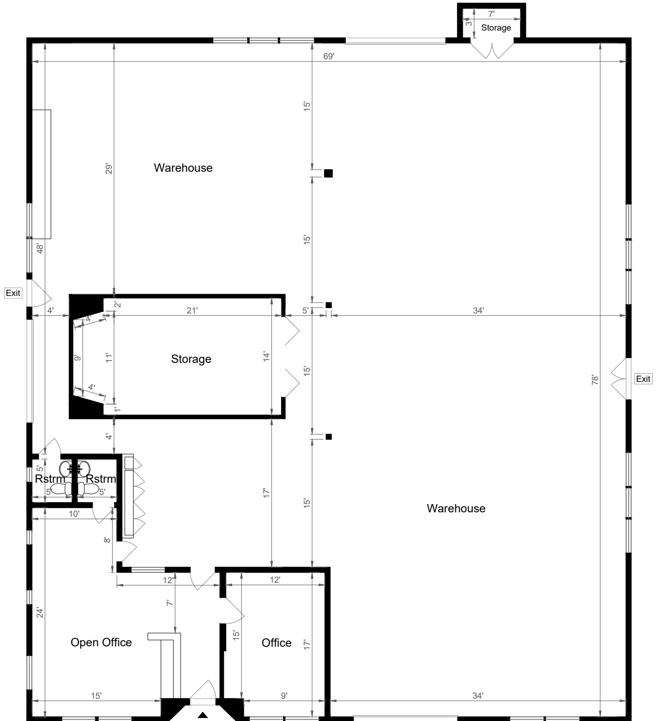
FLOOR PLAN
