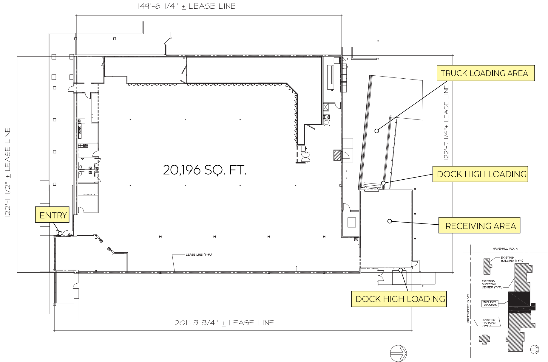
① LEASE OUTLINE PLAN SCALE: 3/32" = 1'-0"
