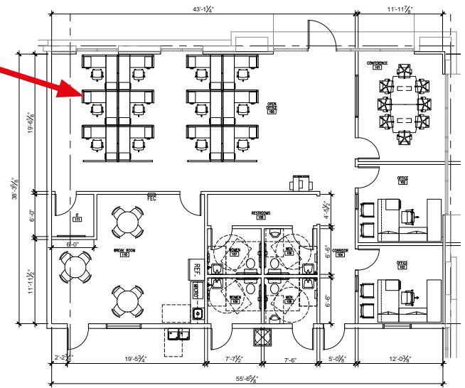
FLOOR PLAN - 2,189 SF
