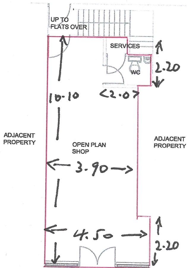
GROUND FLOOR PLAN AS EXISTING SCALE 1:100
