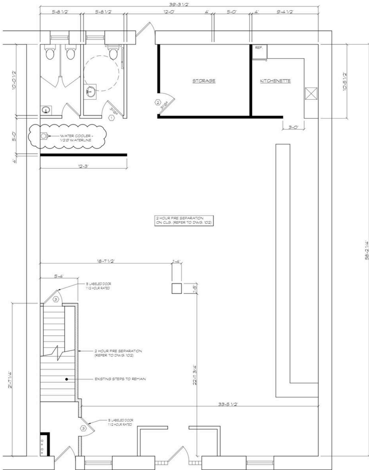
PROPOSED FIRST FLOOR PLAN SCALE 3/8" = 1'-0"
