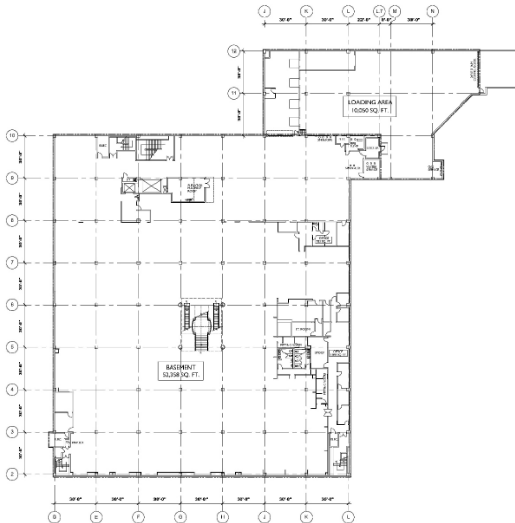
EXISTING BASEMENT FLOOR PLAN
