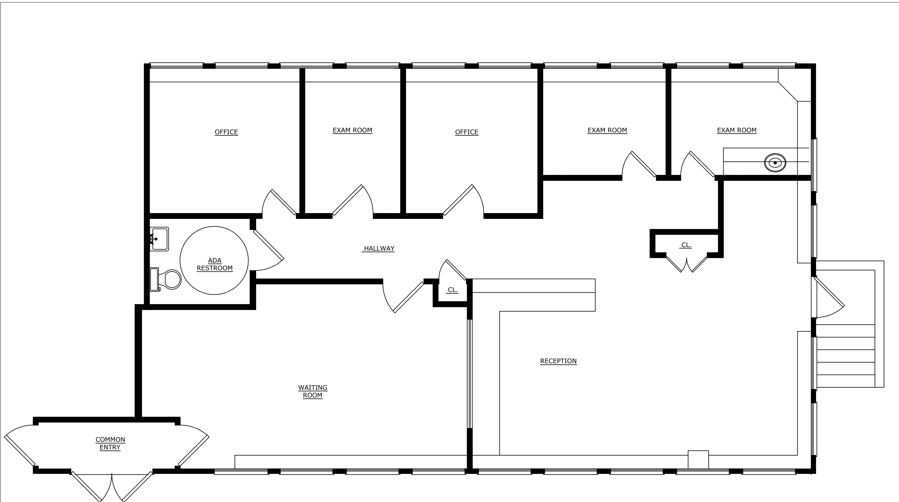
SOUTH BUILDING FIRST FLOOR UNIT C1 = 1,485 S.F.
