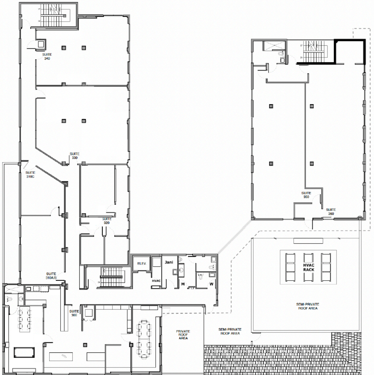
Palm Court Third Floor Plan
