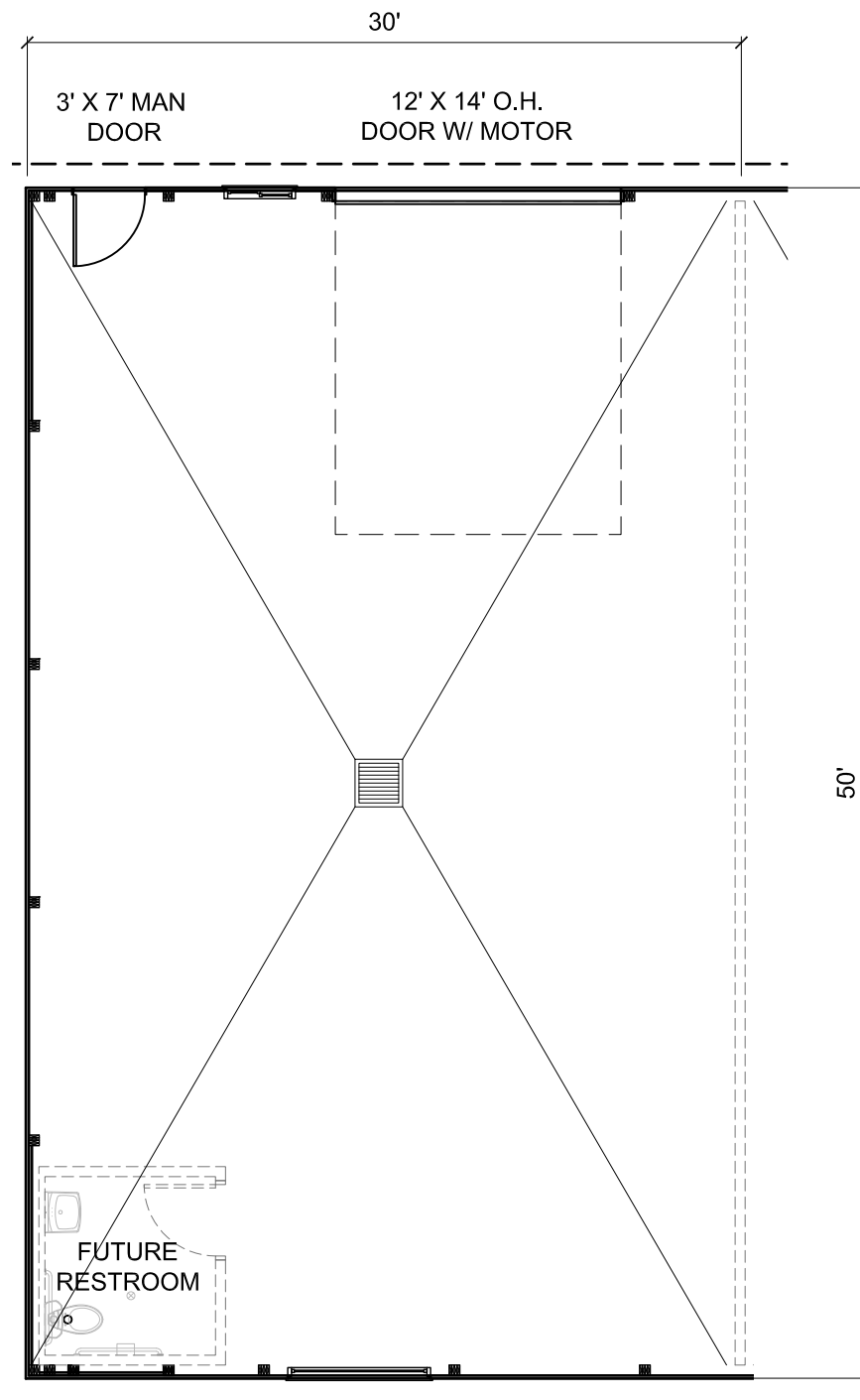
Typical Unit Floor Plan Scale: \frac{1}{8}'' = 1'-0''
