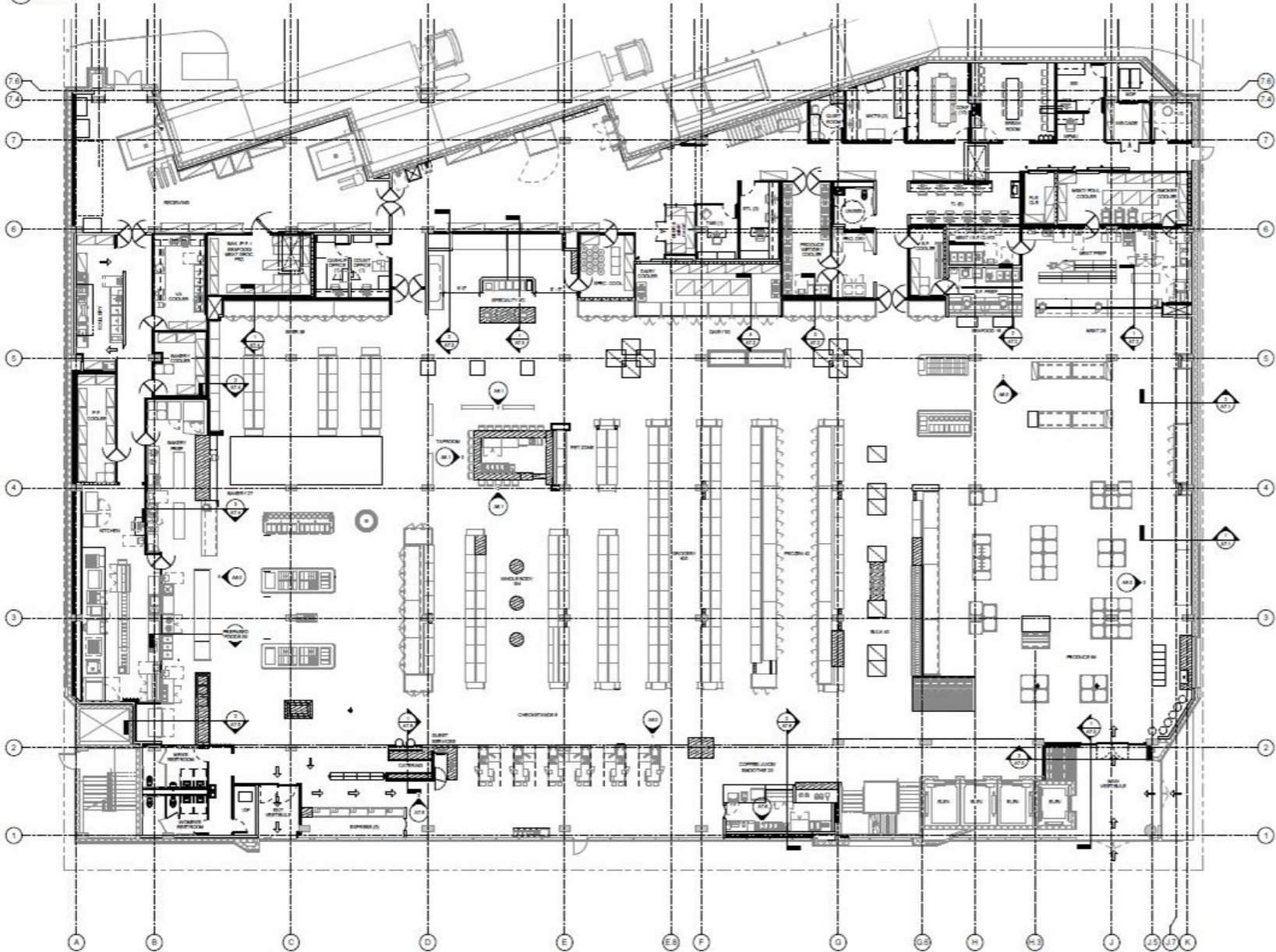
1 FLOOR PLAN - LEVEL 1 - SALES FLOOR 1/8" = 1' 0"
