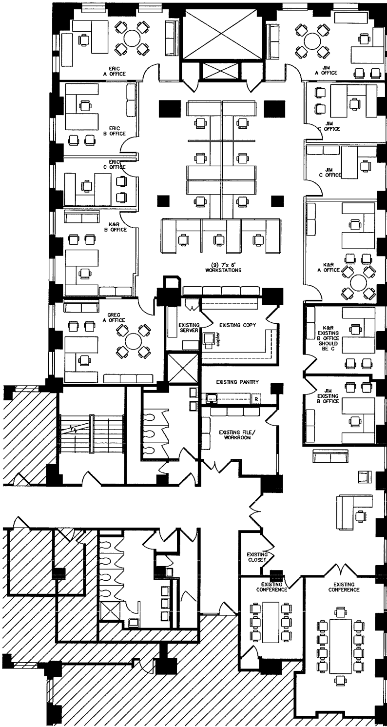
1 SCHEMATIC PLAN SCALE: 3/32" = 1'-0"
