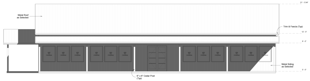
Front Elevation
