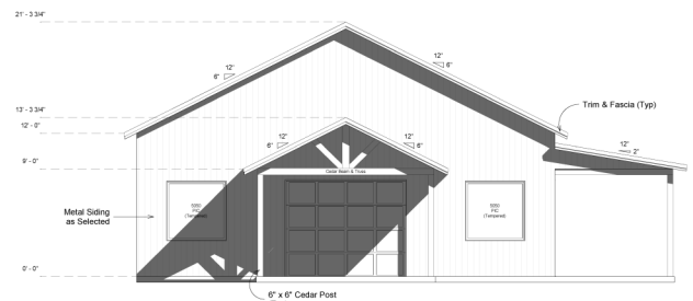
Left Elevation
