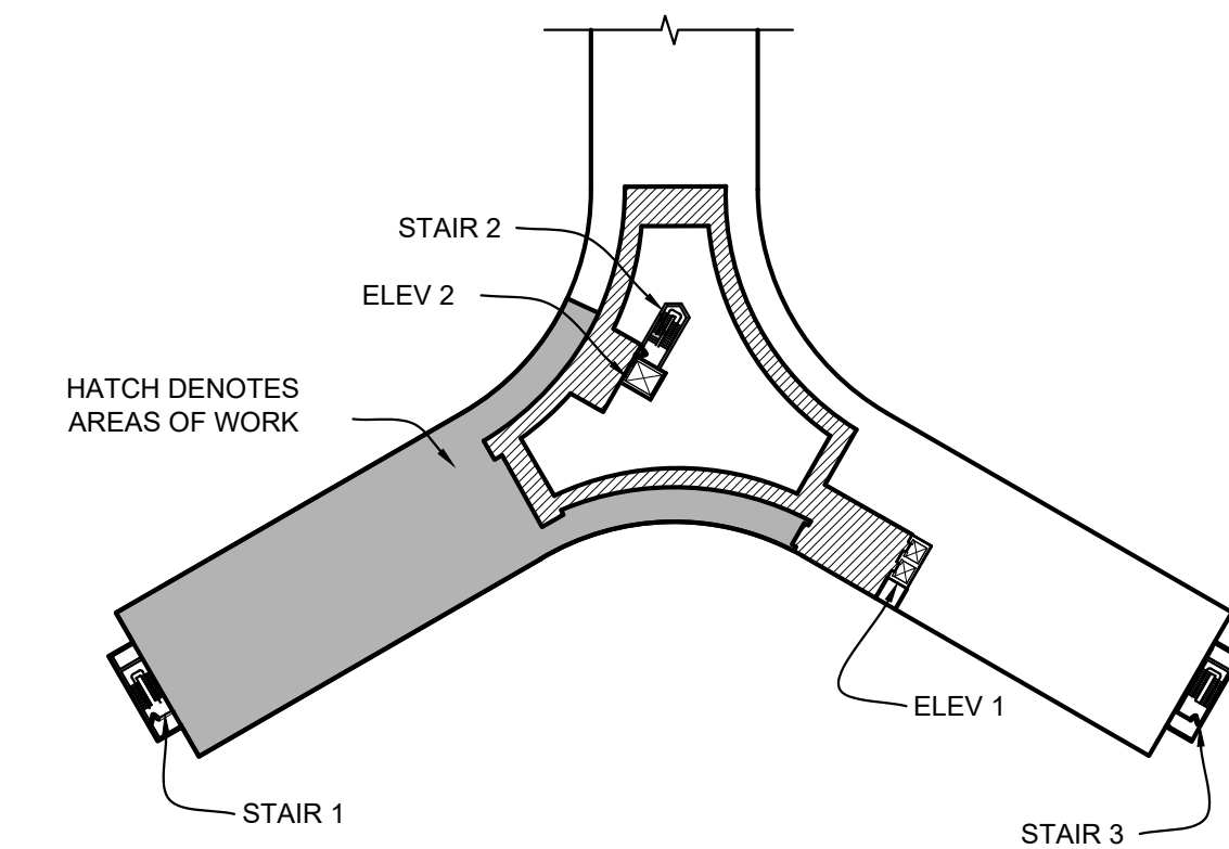
PROJECT KEY PLAN NOT TO SCALE
