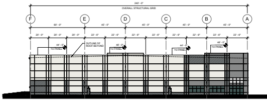
4 EAST ELEVATION
