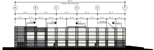
3 WEST ELEVATION
