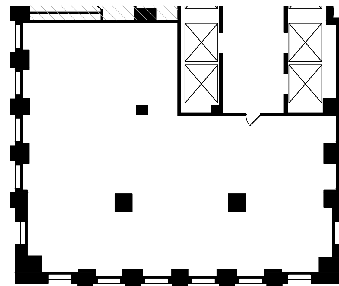
Proposed Demolition Plan - Twenty-Third Floor
