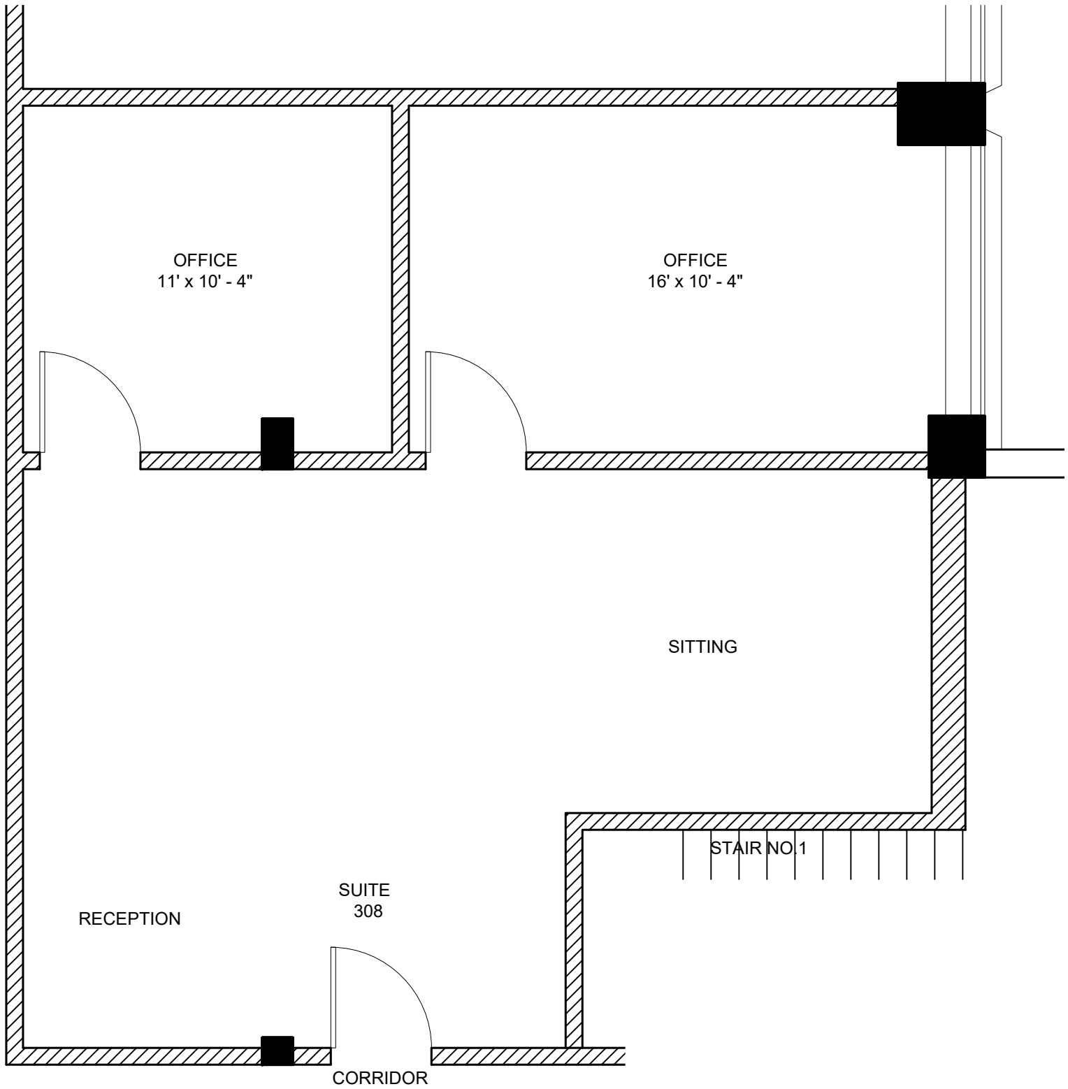
- 3rd FLOOR PART PLAN (SUITE 308) - 1/4" = 1'-0" AREA: 789 R.SQ.FT
