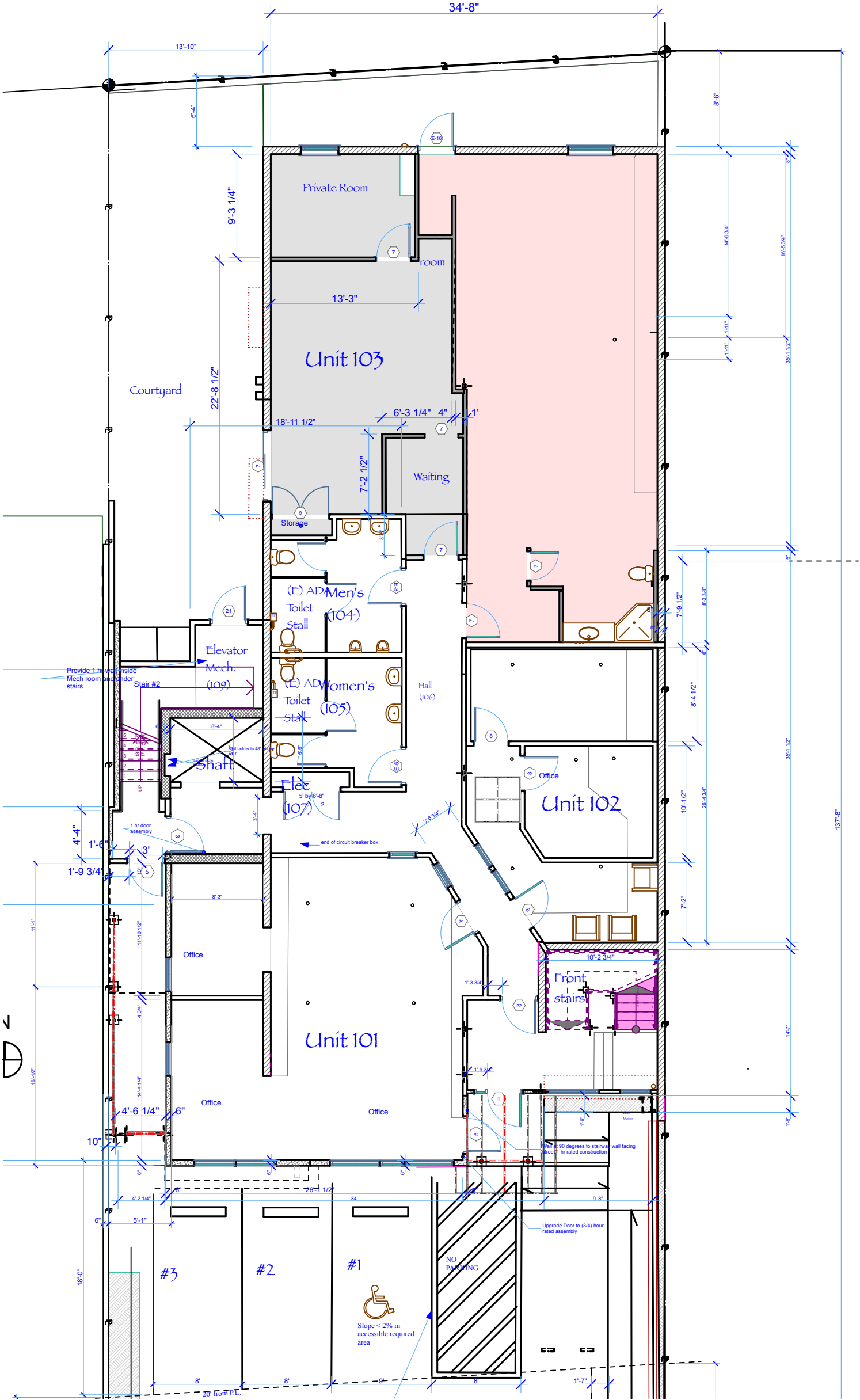
1911 1st Floor Plan
