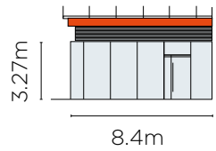
Central Square Elevation - Unit 03
