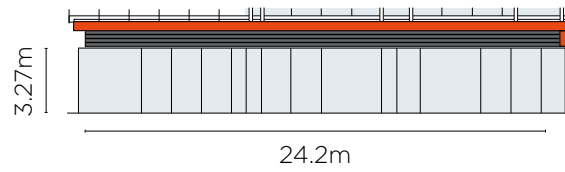
Central Square Elevation - Unit 4
