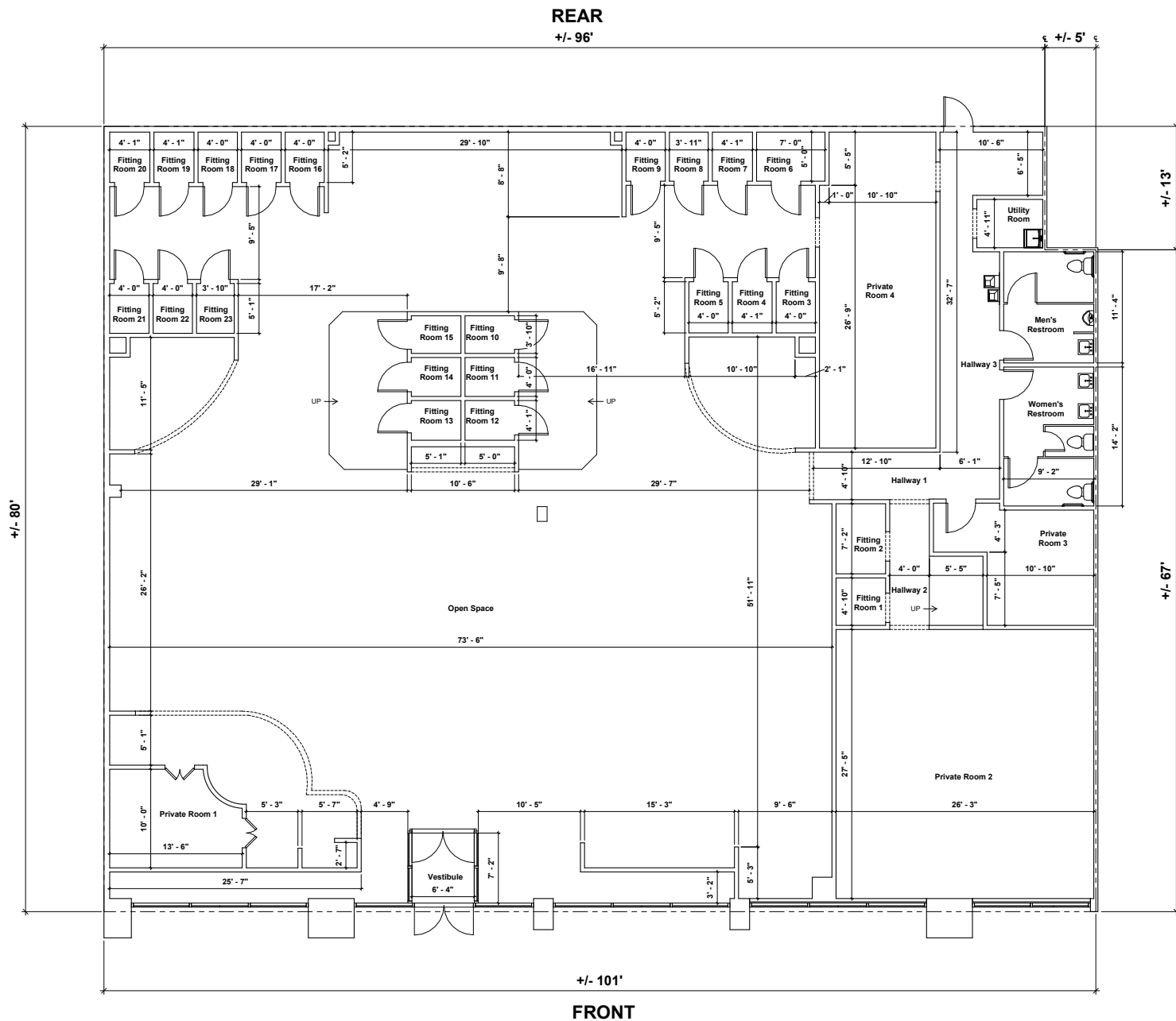
A1 MAIN FLOOR
