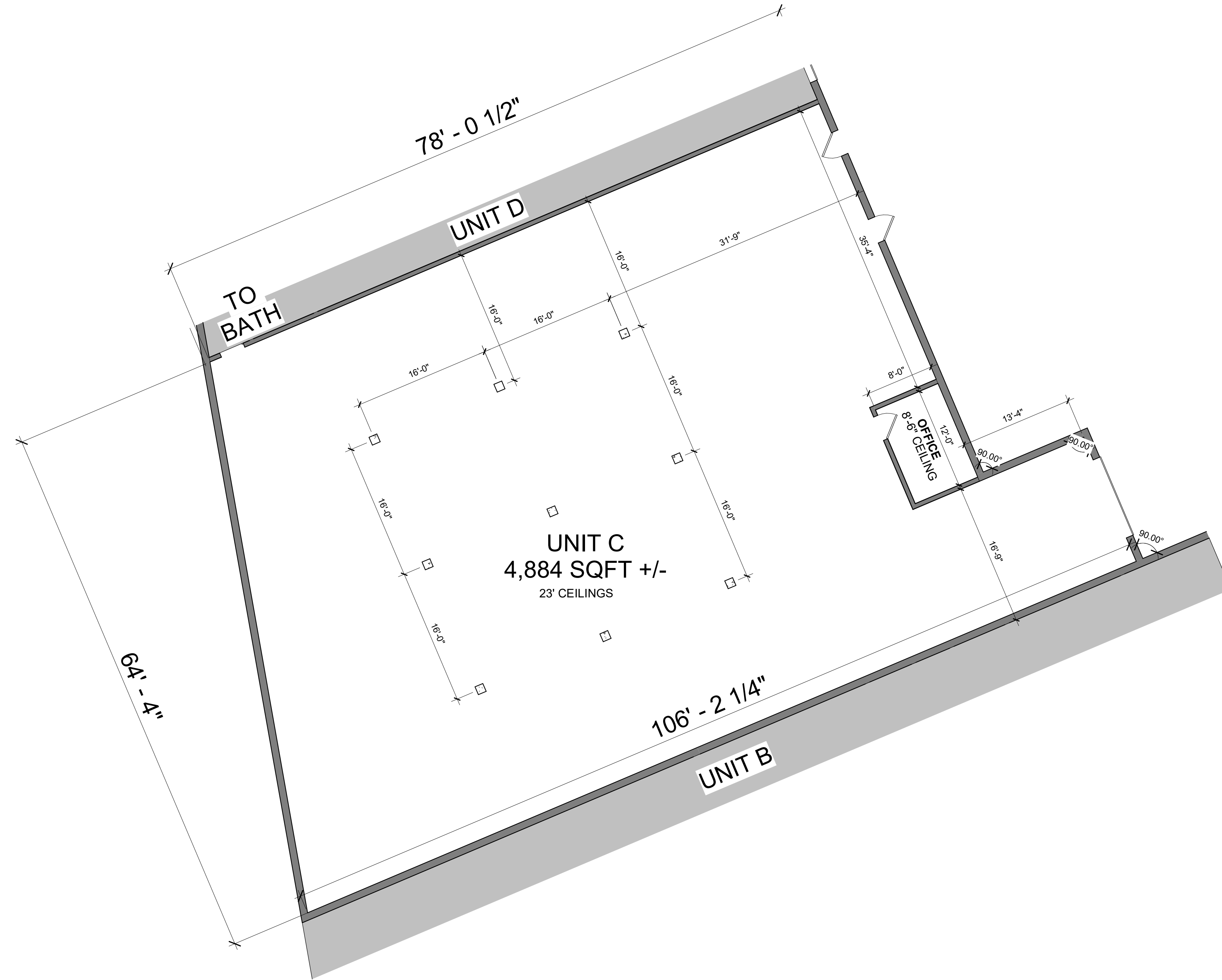
1 UNIT C A1.3 1/8" = 1'-0"
