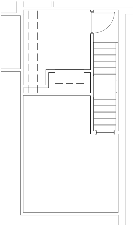
② MEZZANINE 1/8" = 1'-0"
