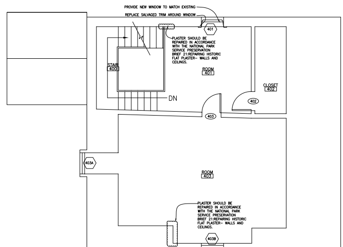
THIRD FLOOR
