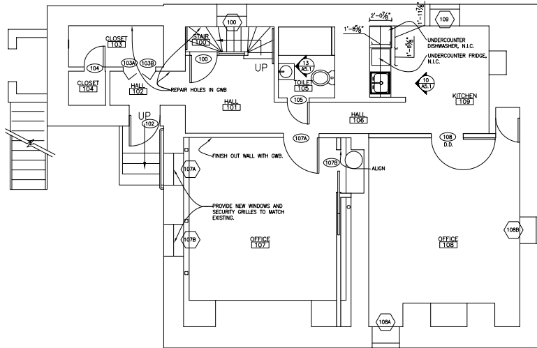
BASEMENT
