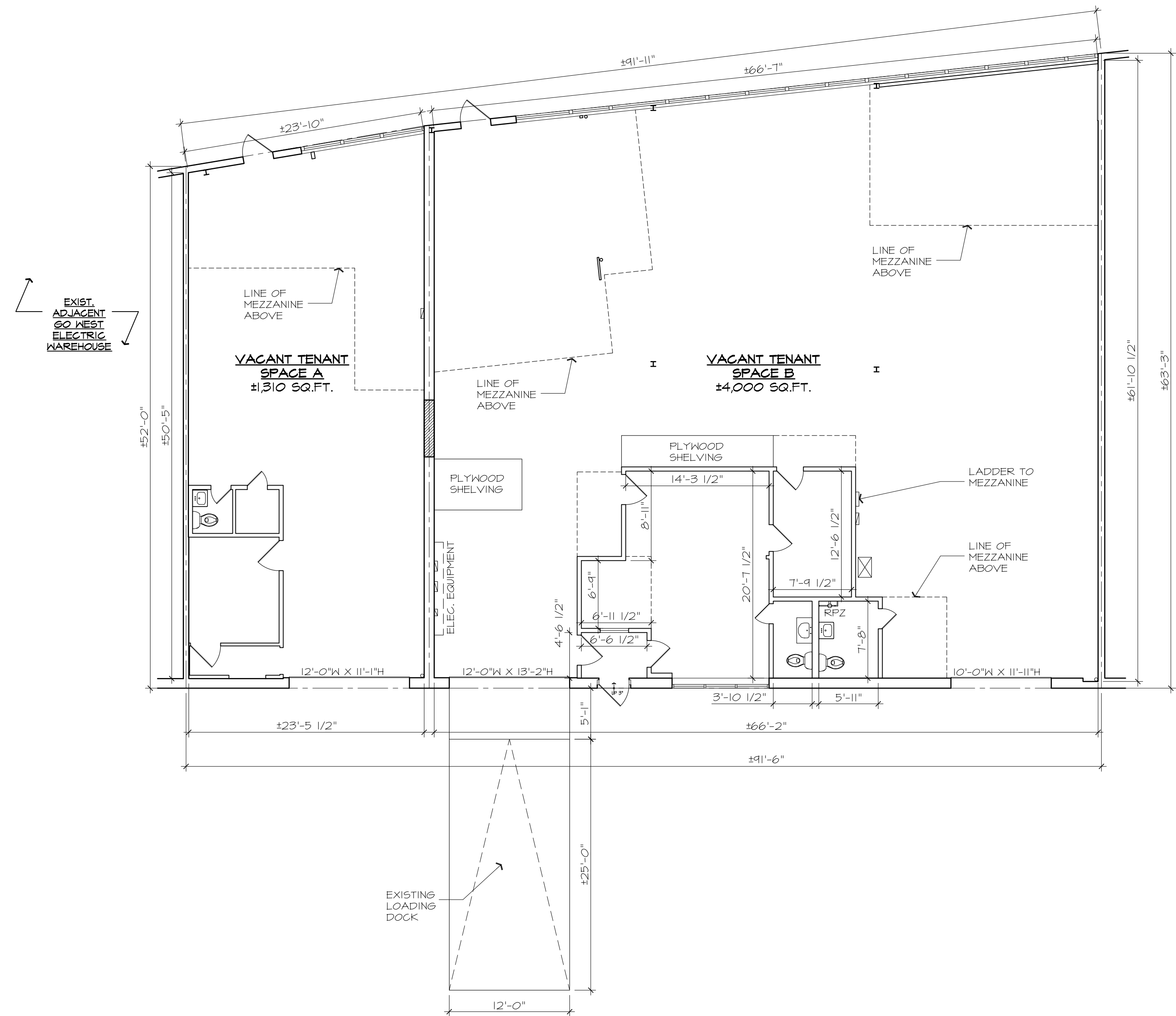
1 LEASE OUTLINE DRAWING SCALE: 1/8" = 1'-0"
