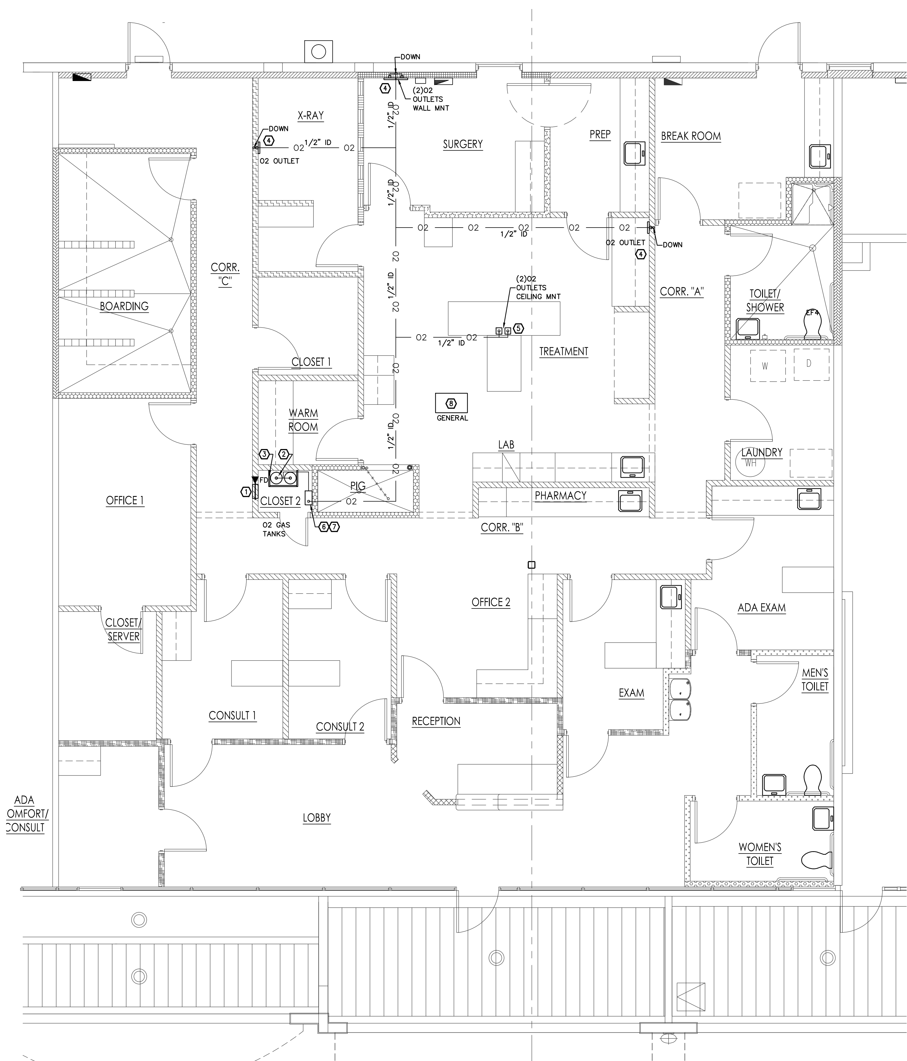
MEDICAL GAS FLOOR PLAN SCALE: 1/4" = 1'-0" PROJECT NORTH
