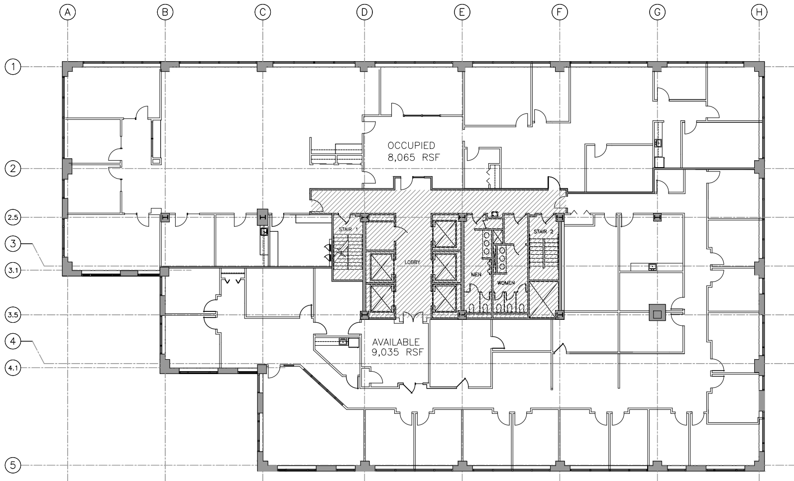
9 9TH FLOOR PLAN SCALE: NONE DATE: 05/06/24
