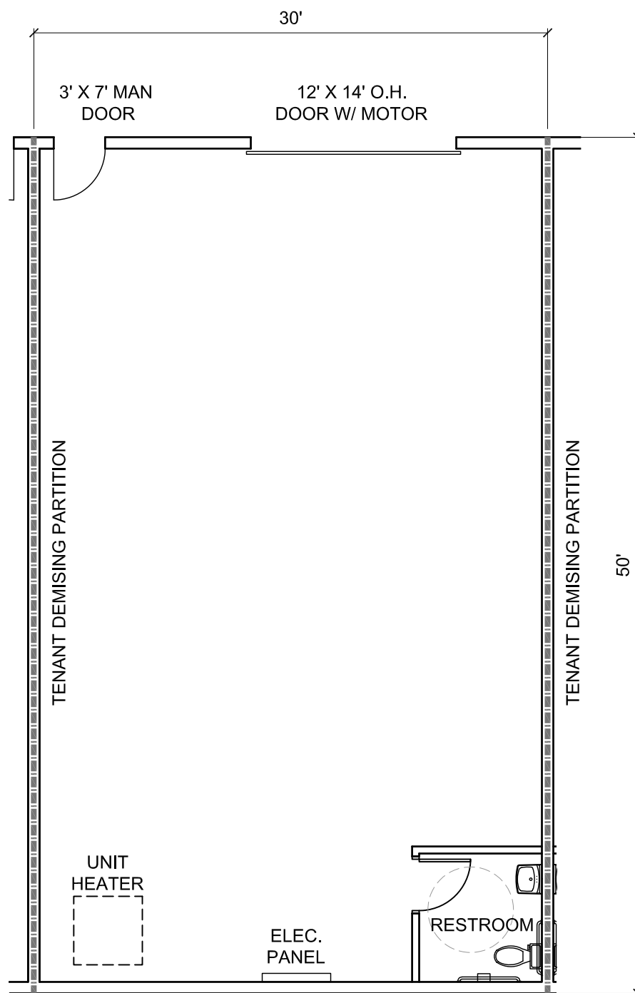
Typical Unit Floor Plan Scale: \frac{1}{8}'' = 1'-0''
