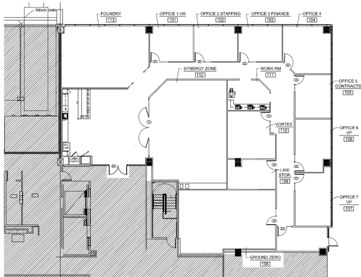
A PARTIAL 1ST FLOOR PROPOSED PLAN SCALE: 1/8"=1'-0"
