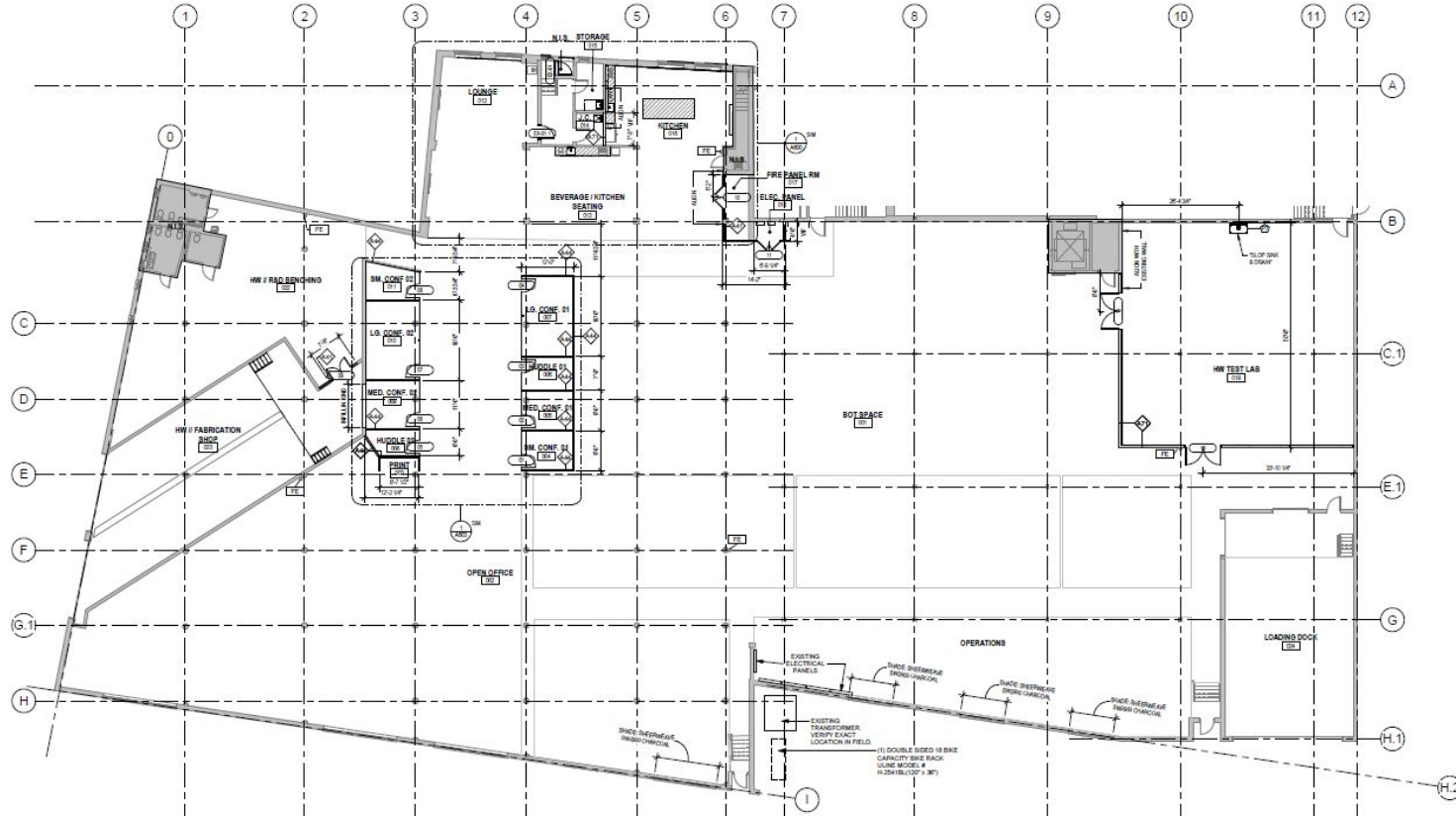
1 WAREHOUSE - OVERALL FLOOR PLAN 3/22/24
