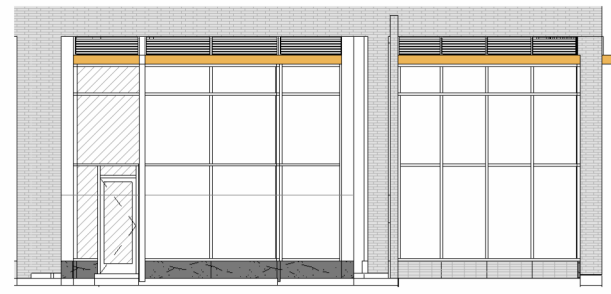
1. East Elevation
