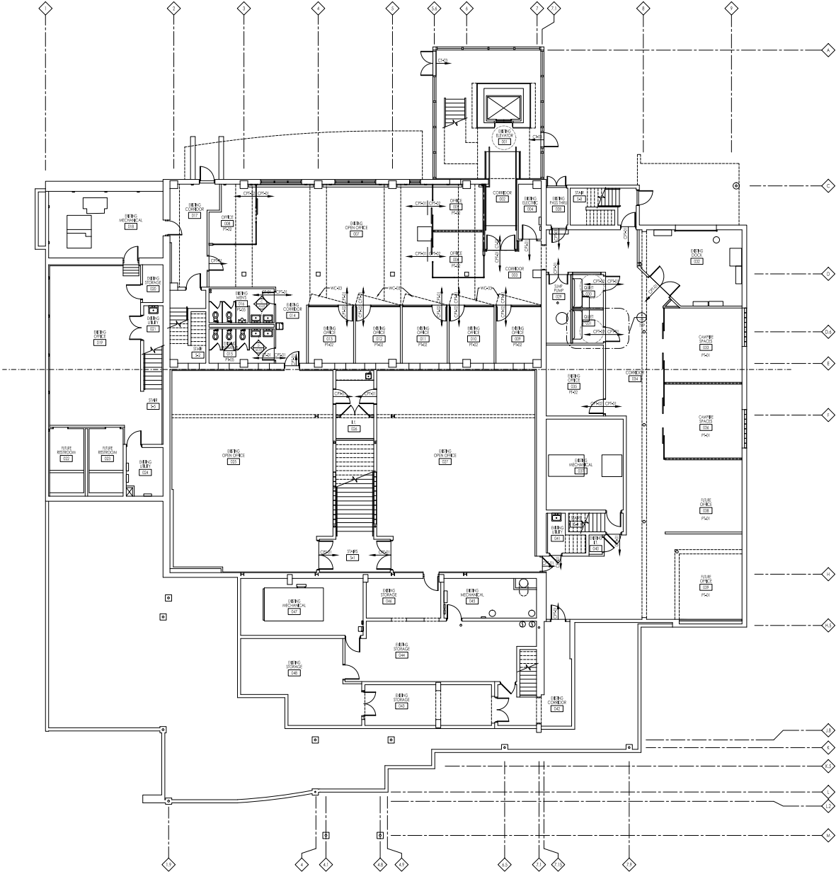
A Proposed Basement Plan
