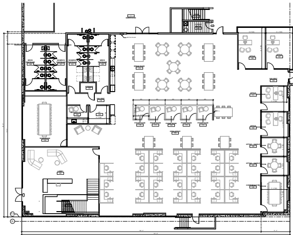
2ND FLOOR PROPOSED PLAN SF ±10,000 SF
