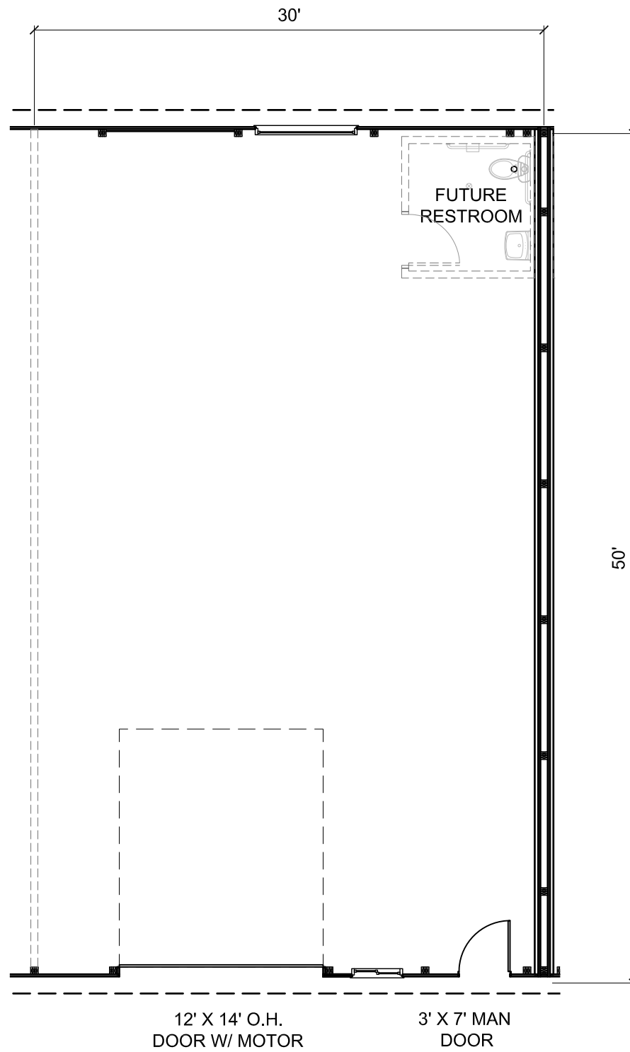
Typical Unit Floor Plan Scale: \frac{1}{8}'' = 1'-0''
