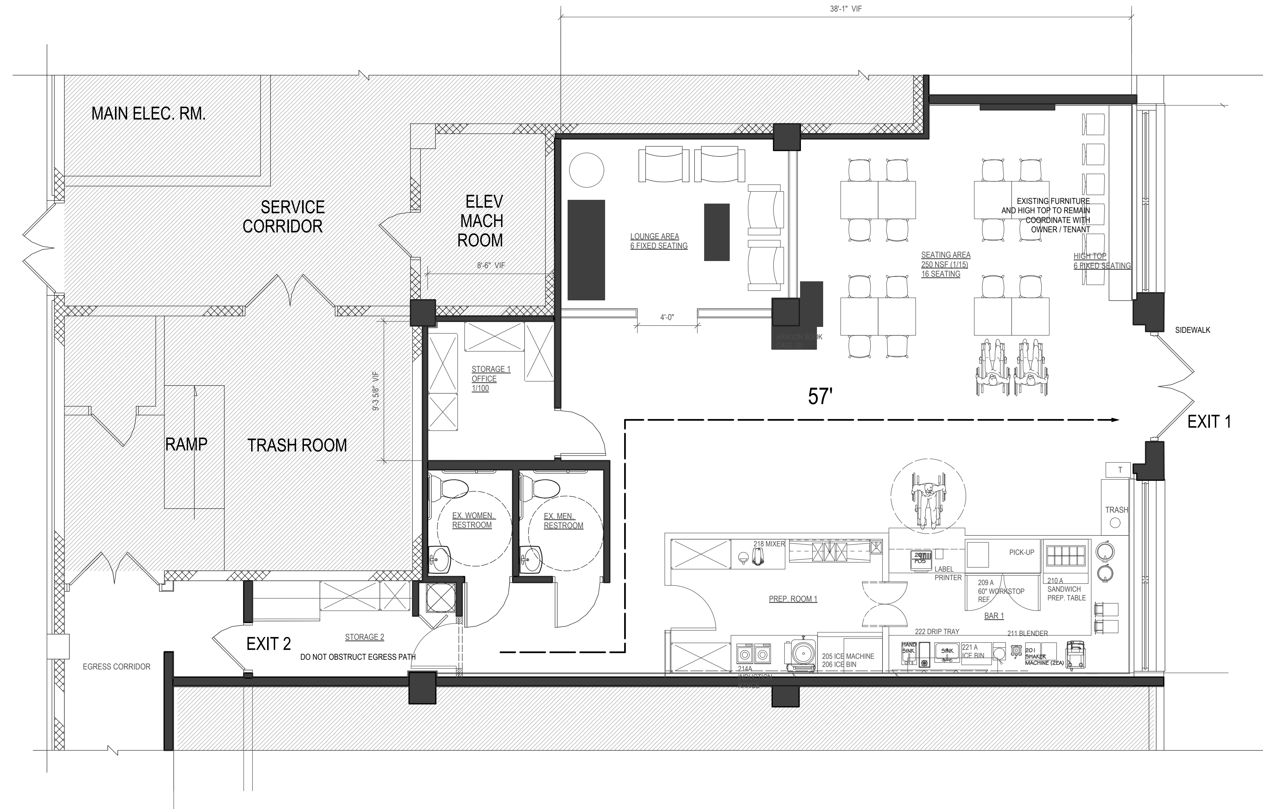
1 A-030 EGRESS PLAN Scale: 1/4" = 1'-0"
