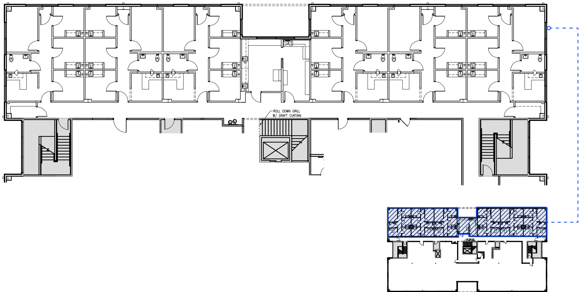
AS-BUILT FLOOR PLAN
