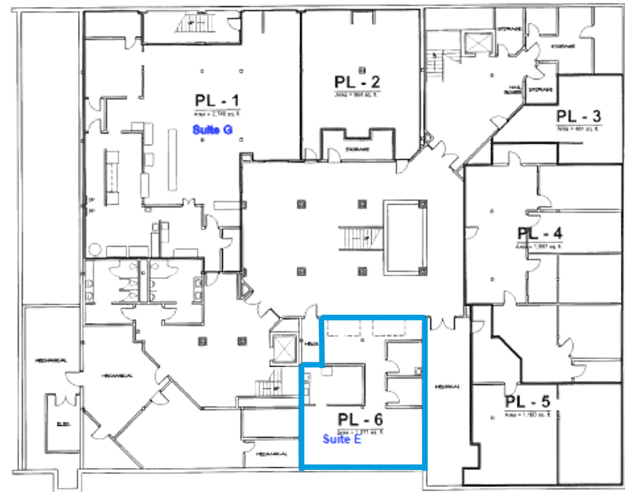
PLAZA LEVEL PLAN SCALE: 1/8" = 1'-0"
