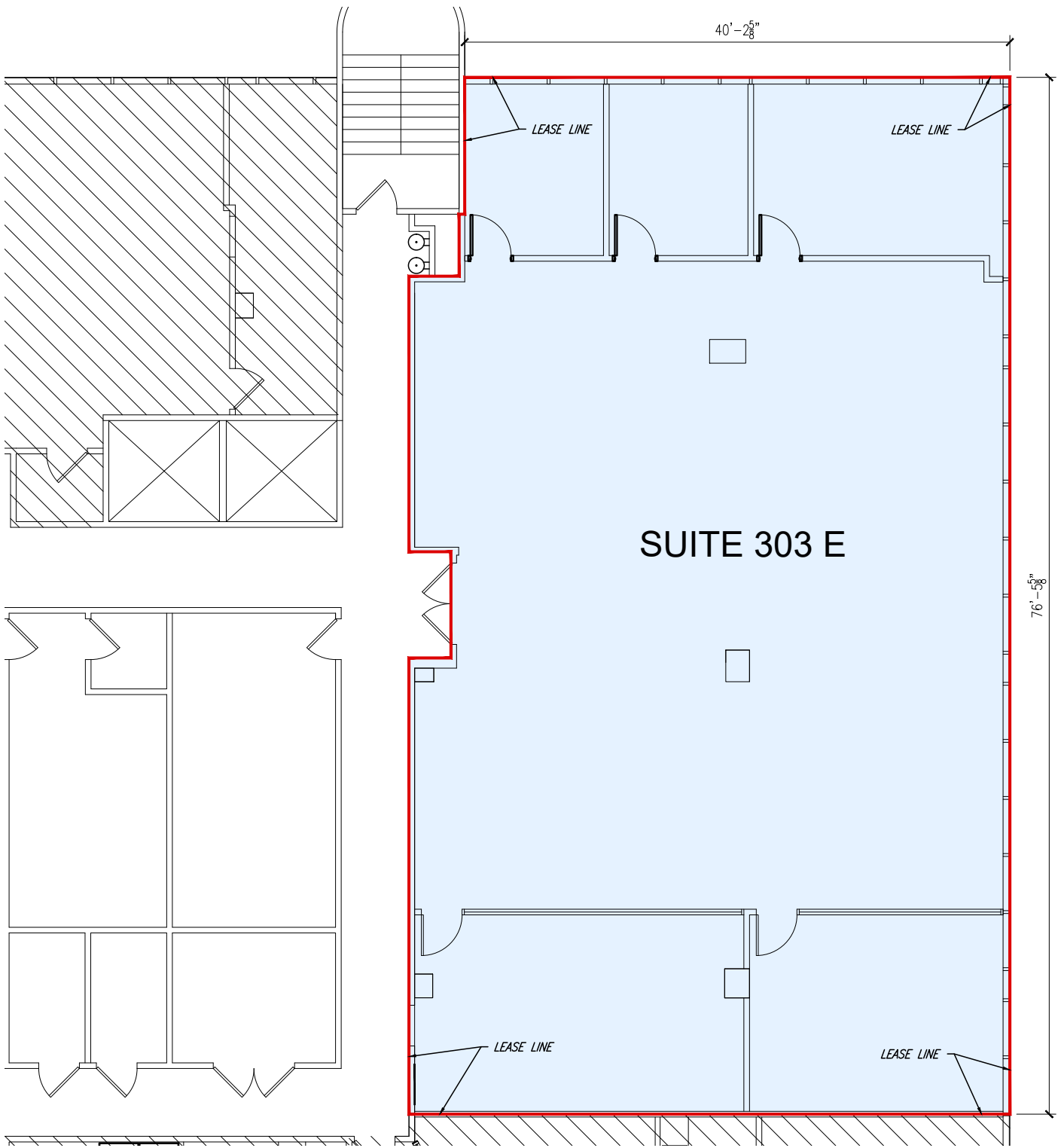
1 FLOOR PLAN SCALE: 3/32" = 1'-0"
