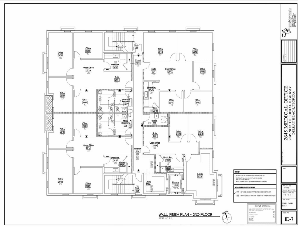
office floor plan upstairs 2645 Delray Professional Building copy
