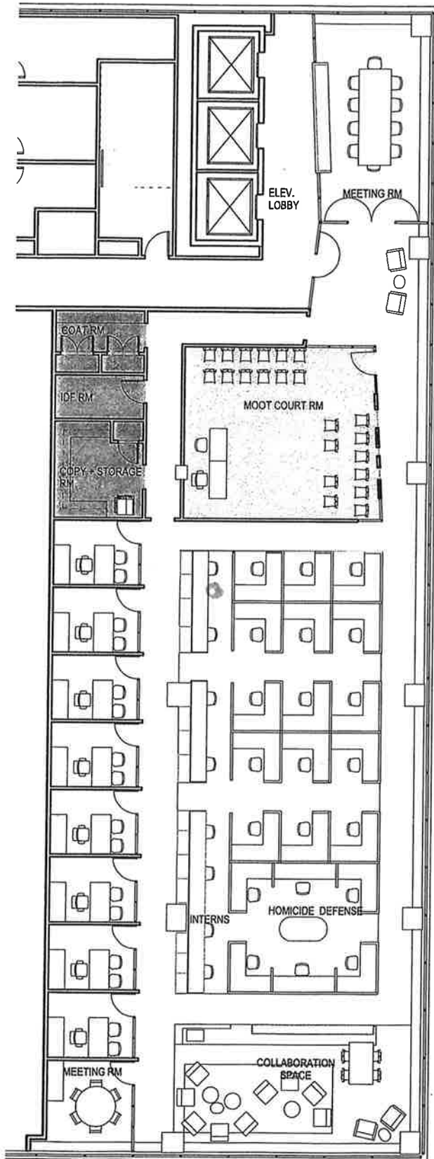
① LEVEL 4 PLAN 3/32" = 1'-0"
