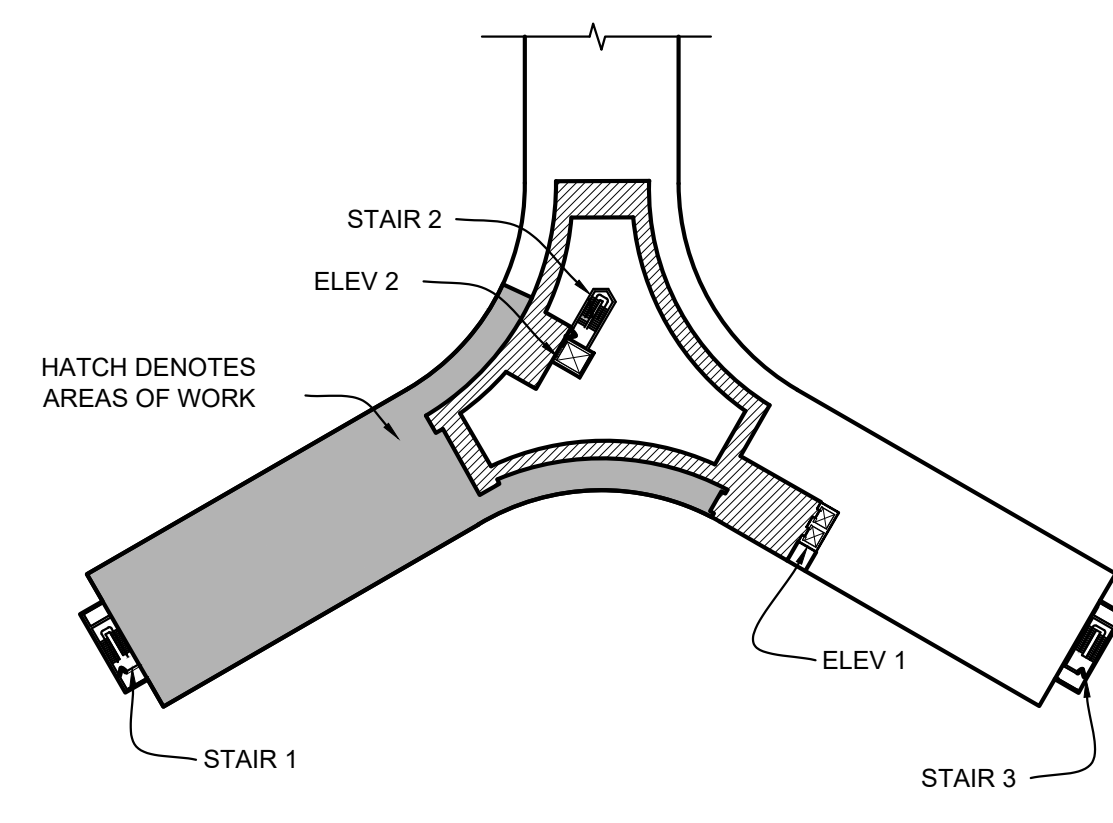
PROJECT KEY PLAN
