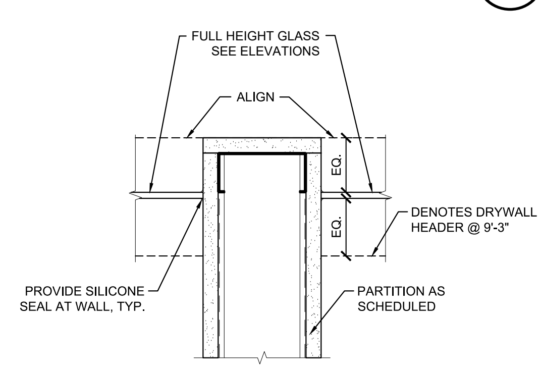
PARTITION @ INTERIOR WINDOW
