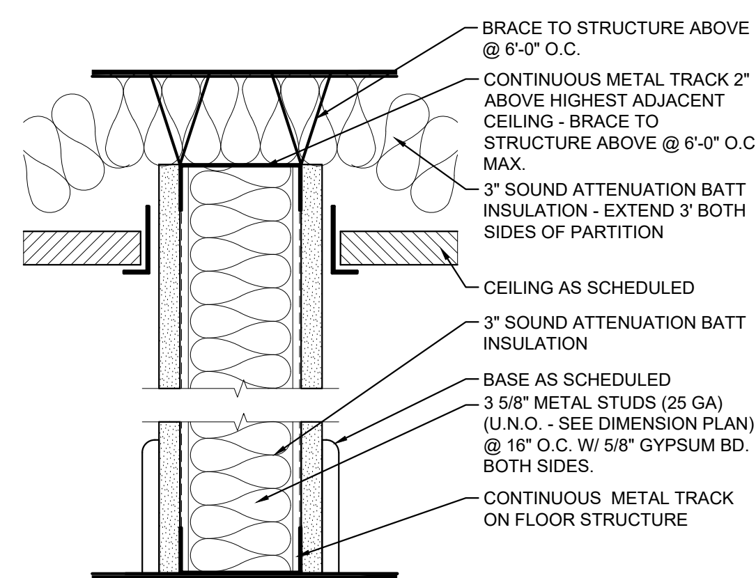
SOUND PARTITION ABOVE CEILING
