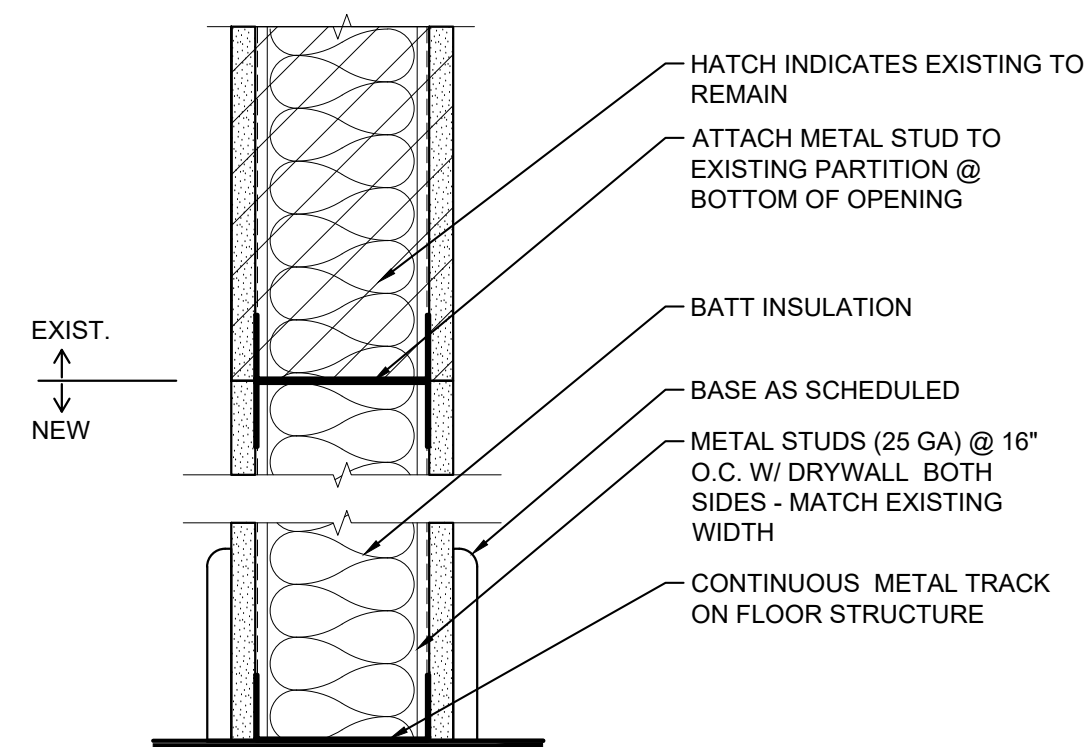
NEW INFILL SOUND PARTITION AT EXISTING WALL OPENING
