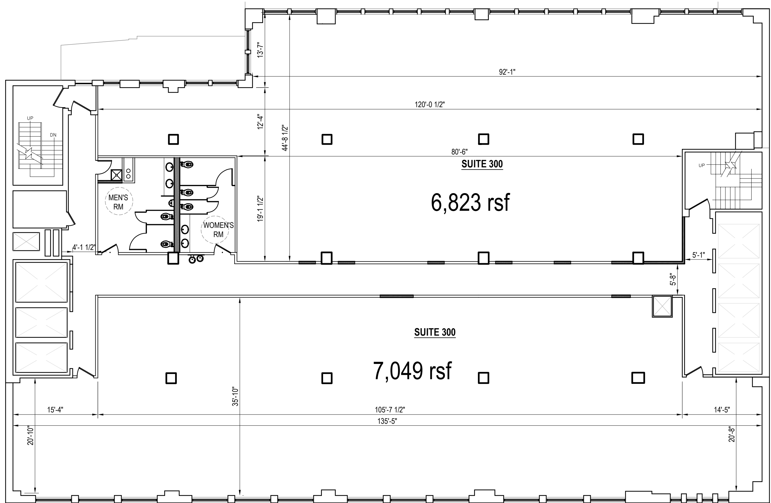
1 150 W30TH ST - 3RD FL DEMISING PLAN SCALE: 3/32" = 1'-0"
