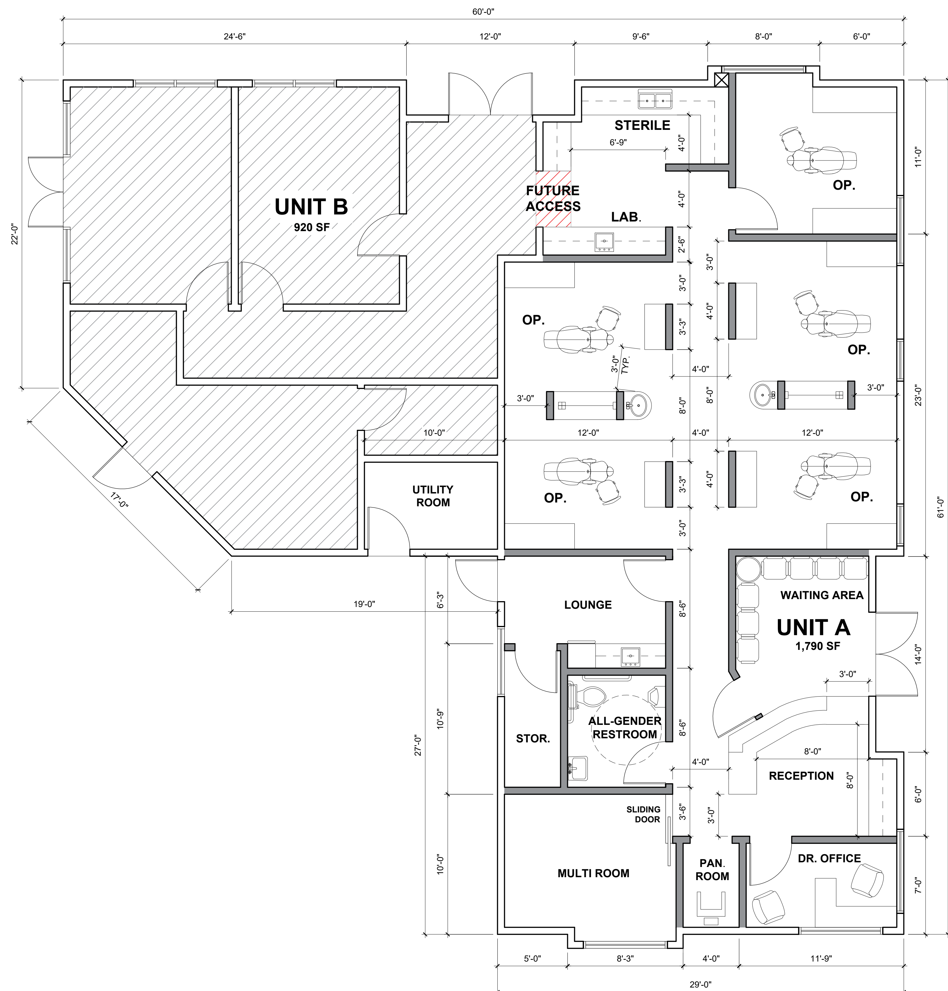
PROPOSED FLOOR PLAN SCALE: 1/4" = 1'-0"
