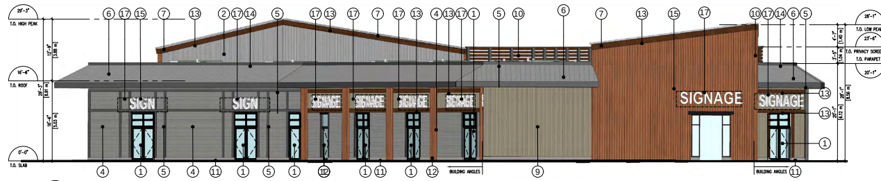
1 NORTH ELEVATION ASIS 1/8"=1'-0"
