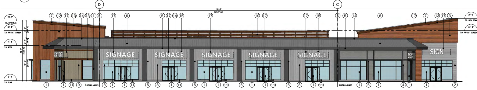
4 WEST ELEVATION ASIS 1/8"=1'-0"
