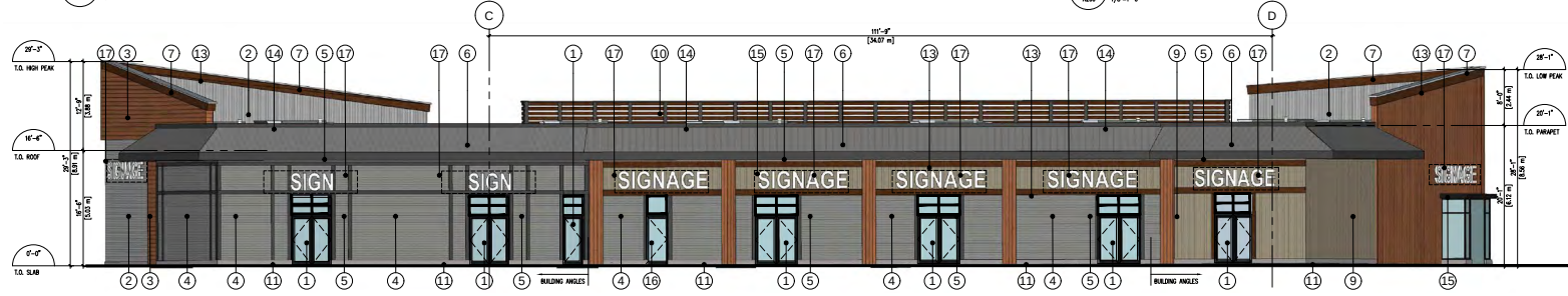
3 EAST ELEVATION ASIS 1/8"=1'-0"
