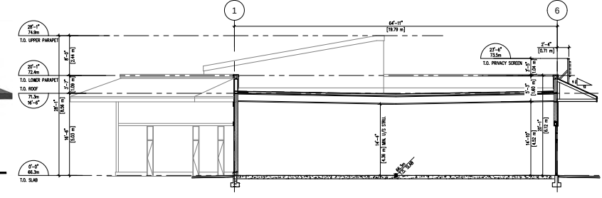
5 BUILDING SECTION ASIS 1/8"=1'-0"
