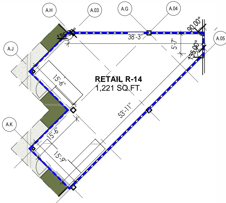
2 RETAIL SPACE - R14 LOD SCALE: 1/16" = 1'-0"
