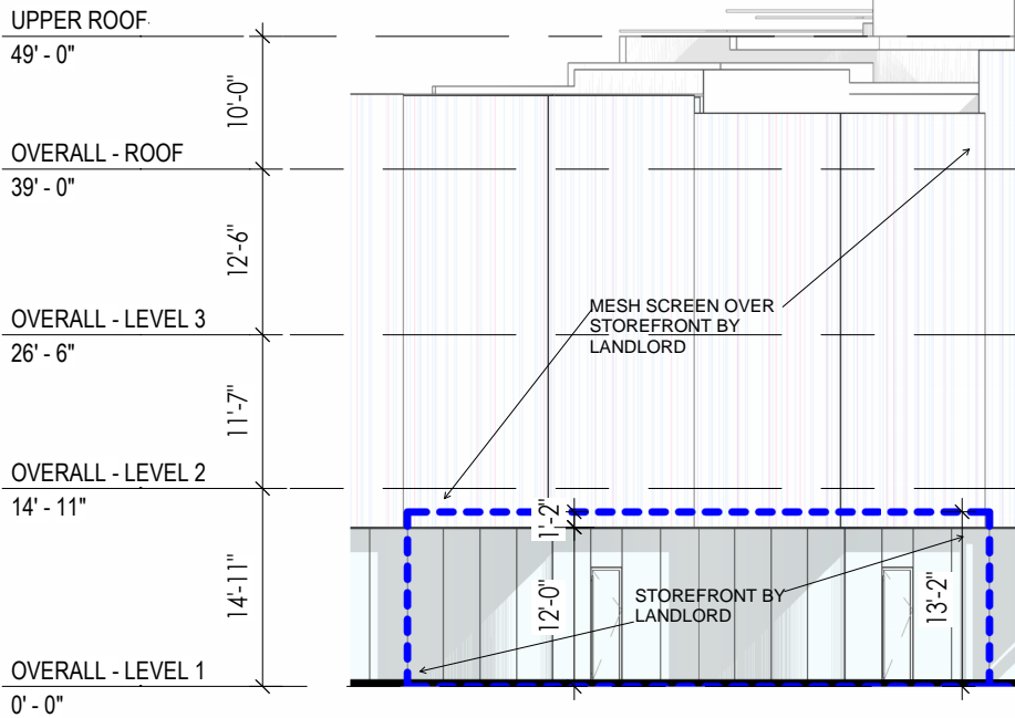
3 SOUTH ELEVATION - RETAIL R14 LOD SCALE: 1/16" = 1'-0"
