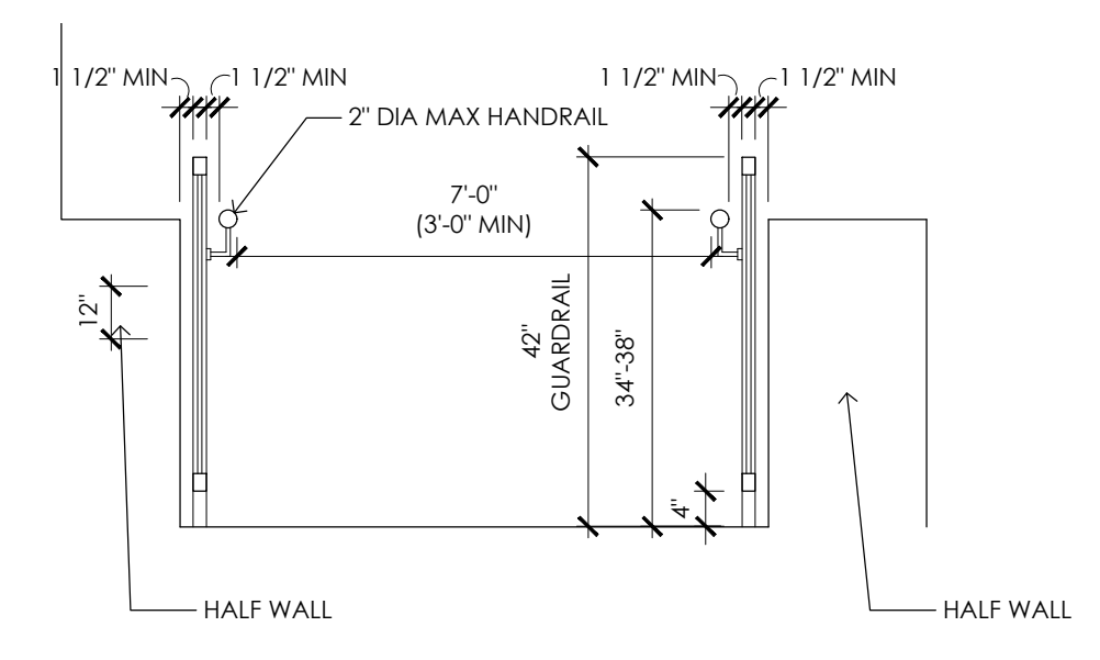
2 SECTION AT ADA RAMP SCALE: 1/2" = 1'-0"
