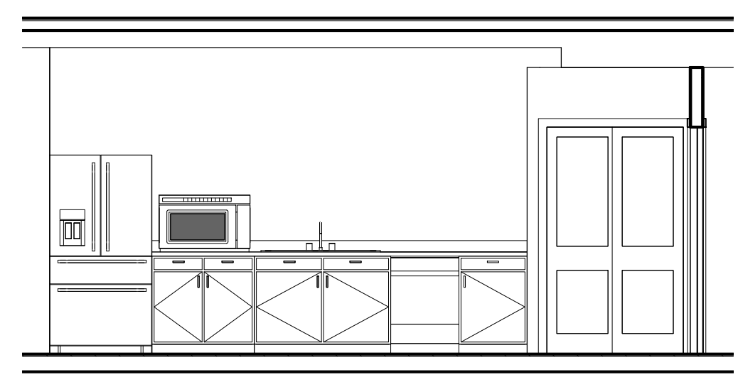
3 Kitchenette 1/4" = 1'-0"
