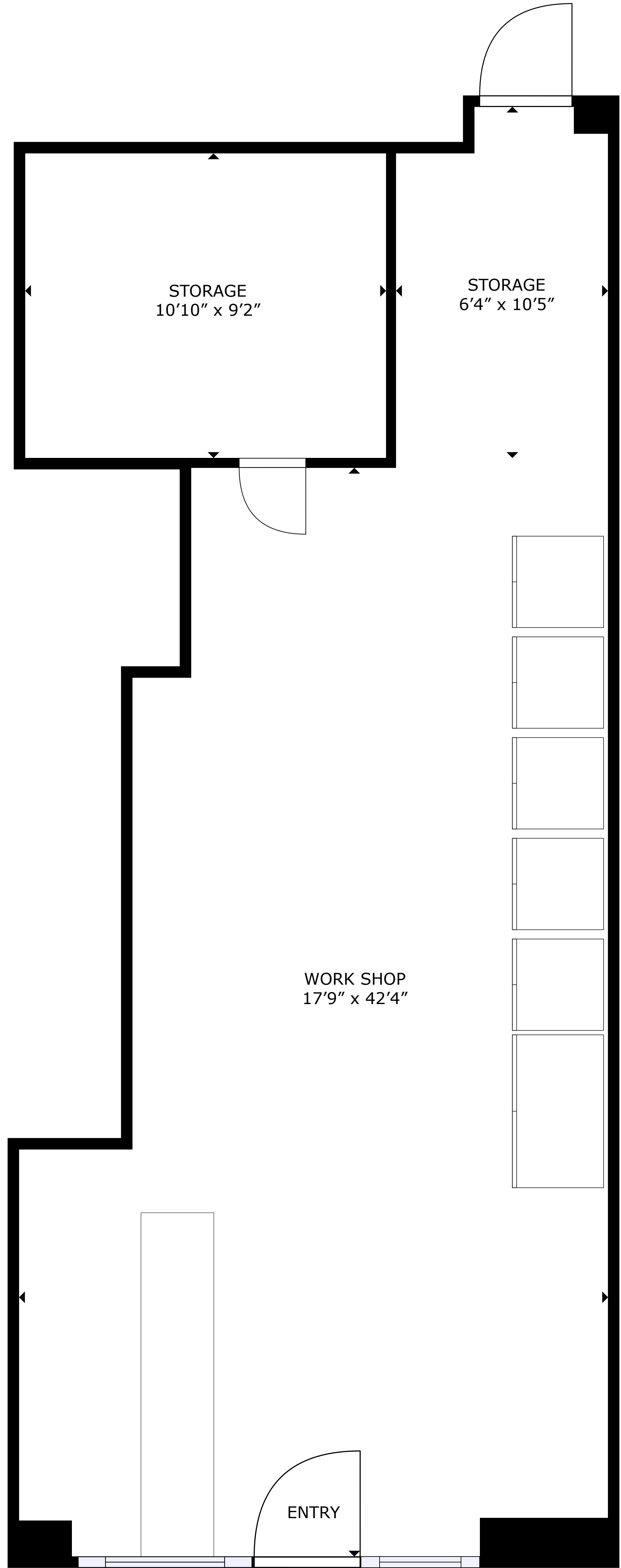
FLOOR PLAN
