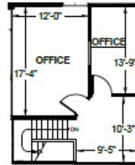
MEZZANINE
