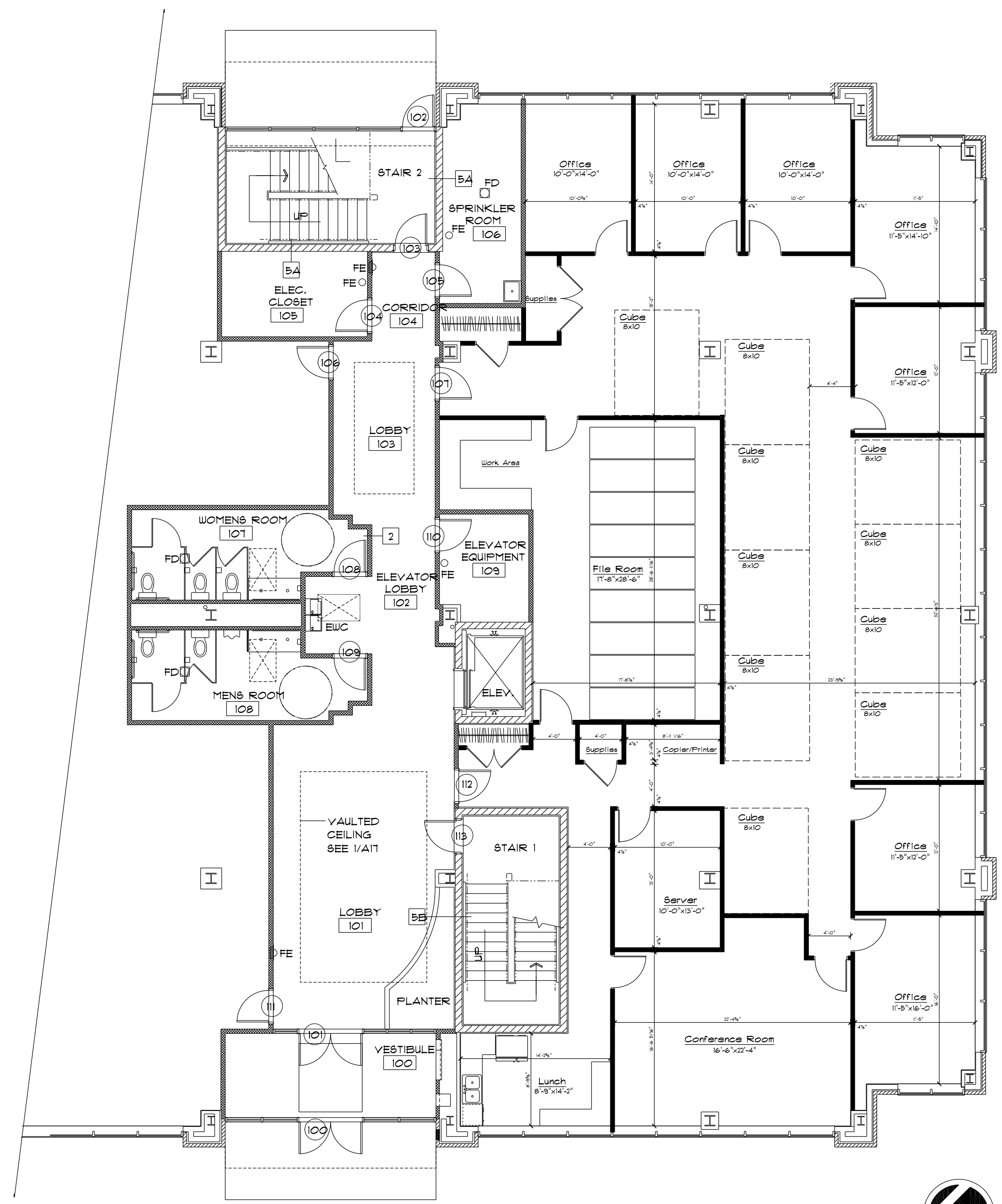
Part. First Floor Plan
