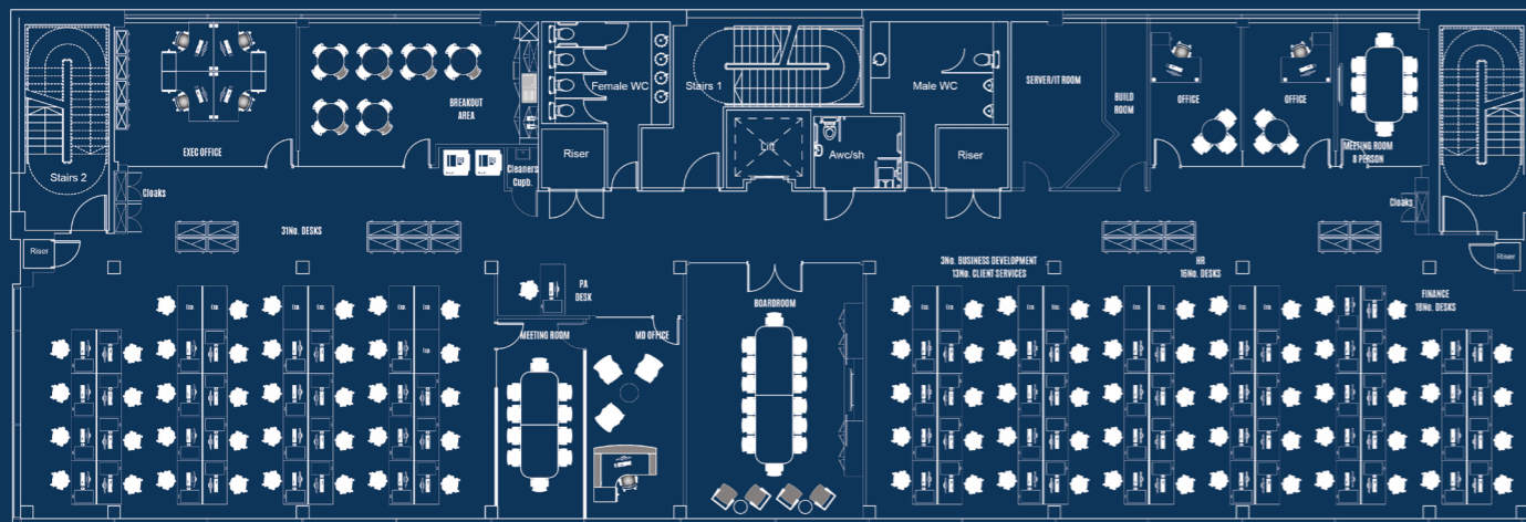
PROPOSED FIRST FLOOR
