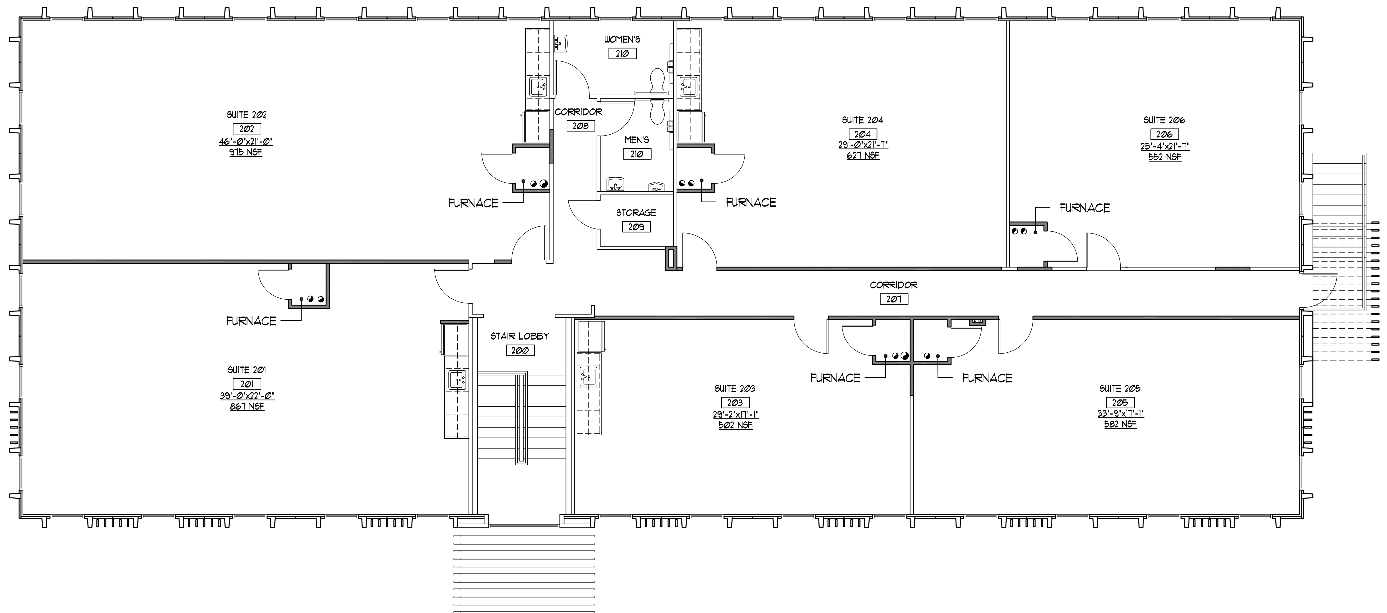
1 SECOND FLOOR PLAN 1/4" = 1'-0"
